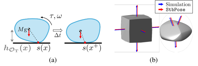
Fig. 4: (a) Illustration of an object settling on a flat surface during \Delta t , with red arrows showing x and x^+ in (8), in the global frame. (b) Comparison plot of the physics simulation and StabPose for a cube and an arbitrary shape, with a small offset added to the arrows for clarity.
